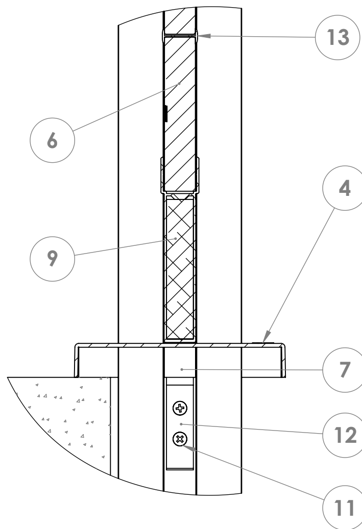
DETAIL C SCALE 1 : 5
